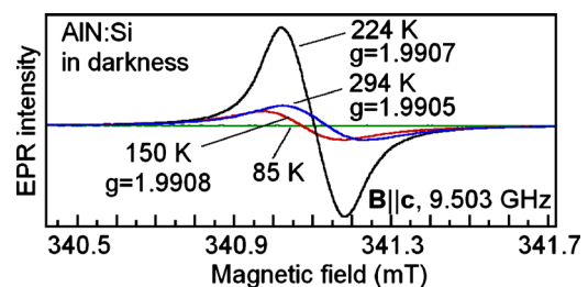
FIG. 1. (Color online) EPR spectra of the shallow Si donor in unintentionally Si-doped AlN measured in darkness for B||c at different temperatures during cooling down the sample. The EPR signal is disappeared when cooling the sample to \sim 85 K in darkness. A small shift in the EPR line to lower magnetic fields is due to the temperature dependence of the g -value of the shallow donor.
