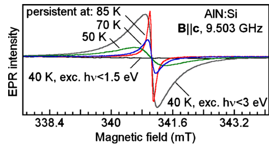
FIG. 3. (Color online) EPR spectra at 40 K under illumination with different photon energies and the persistent signals in darkness at different temperatures measured with the microwave power of 1 mW and a field modulation of 0.03 mT.
