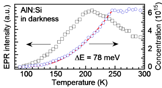
FIG. 2. (Color online) Temperature dependence of the EPR intensity (double integrals) of the shallow donor signal (open squares) in AlN measured in darkness with microwave power of 1 mW and the corresponding concentration on the shallow d^0 level (open circles) assuming a uniform doping in the sample. The solid curve represents the fits using Eq. (1).
